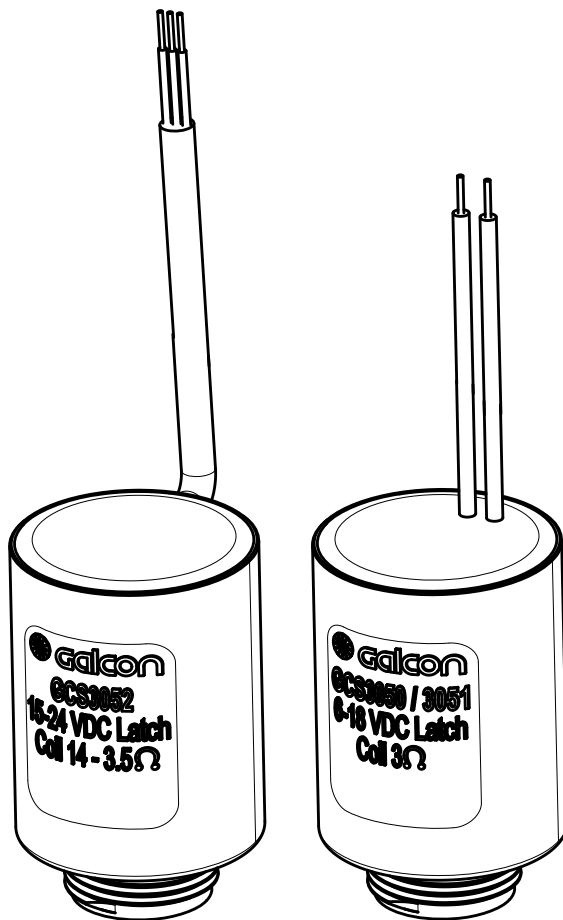
S1603 3 Wire
